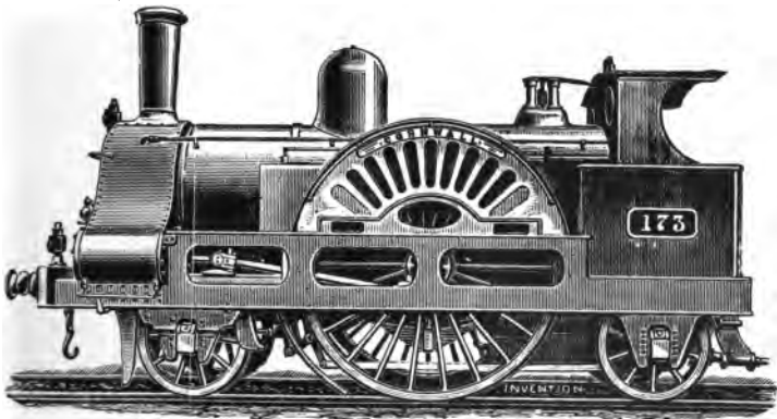
Fig. 58.—"Cornwall," London and North-Western Railway, 1863 to 1903 (Now, No. 3020.)
